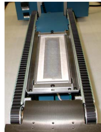
Lower Heater Assembly with Side Heat Shields
