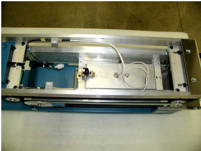
Top Heater Assembly with Over-temp Switch
